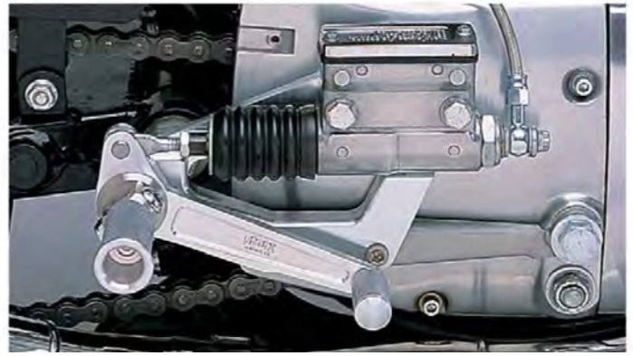
1991-2003 right side brake (low pipe)
