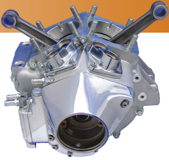
Shovelhead 80" Short Block V-Twin short block is shipped fully assembled and a Manufacturer Statement of Origin is supplied.
