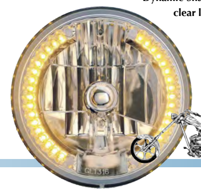
7" Headlamp 5 3/4" Candle Power in 60/55w and 7" also available in 100/55w
