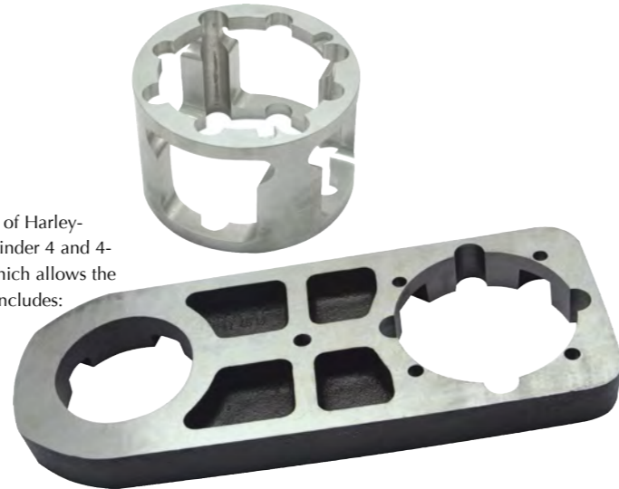
Replacement Polished Billet Oil Pump body
