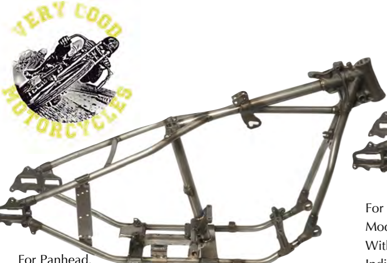
For Panhead. Model year 1948 with neck 30° "Wishbone" With German TÜV certificate Individual requests are possible
